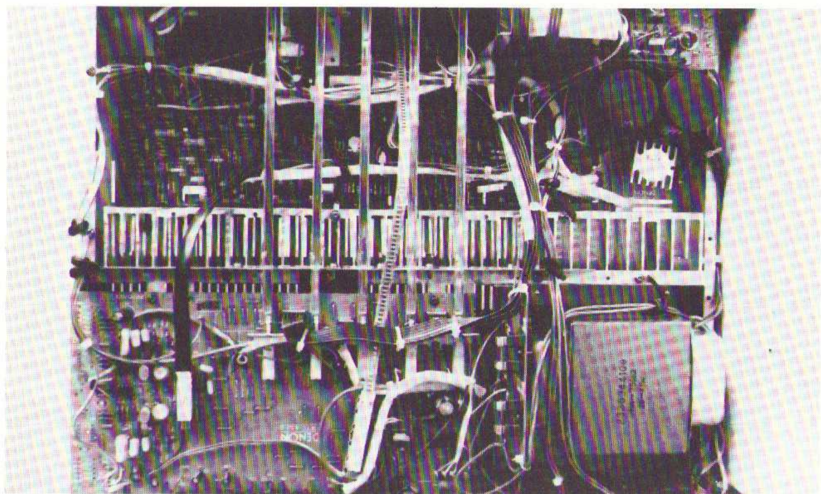
HARMAN KARDON PM-650
